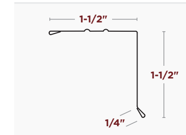
1-1/2"x1-1/2" STYLE A ROOF EDGE (AVAILABLE WITH EMBOSSING)
