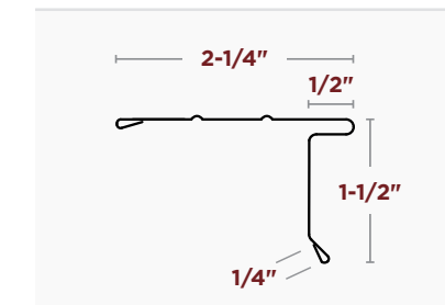
4-1/2" STYLE SR ROOF EDGE
