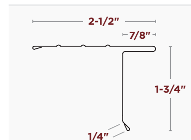
5-1/2" STYLE L ROOF EDGE
