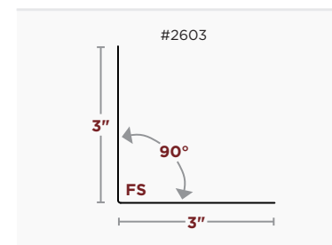
4"x5" INSIDE ANGLE FLASHING (90 DEGREES)
