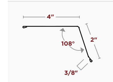
2"x4" GUTTER APRON WITH HEMS
