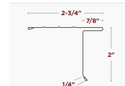
6" STYLE LL ROOF EDGE
