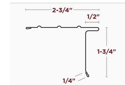
5-1/2" STYLE SRLL ROOF EDGE
