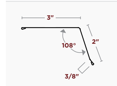
2"x3" GUTTER APRON WITH HEMS
