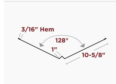
24" STYLE W FORMED VALLEY WITH HEMS 10'
