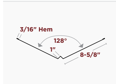
20" STYLE W FORMED VALLEY WITH HEMS 10'
