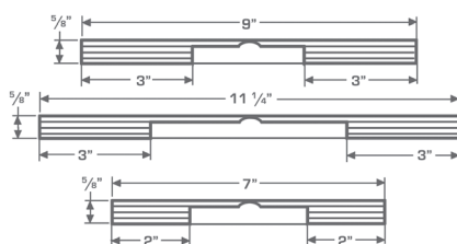
CraftGrade Ridge Vents Low Profile - End Views
