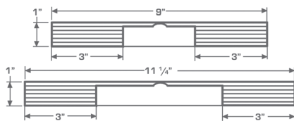
CraftGrade Ridge Vents High Profile - End Views
